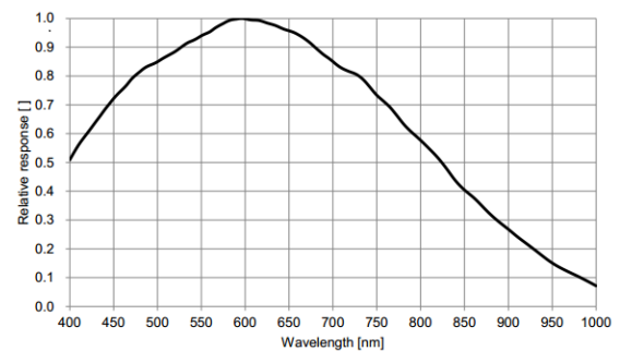
MV-CH120-10UM V5
