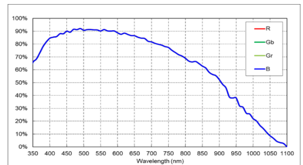
MV-CH050-60UM
